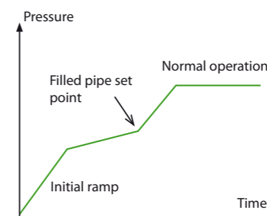
Pipe Fill Mode to prevent water hammering
